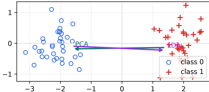
PCA and LDA find the same useful direction
