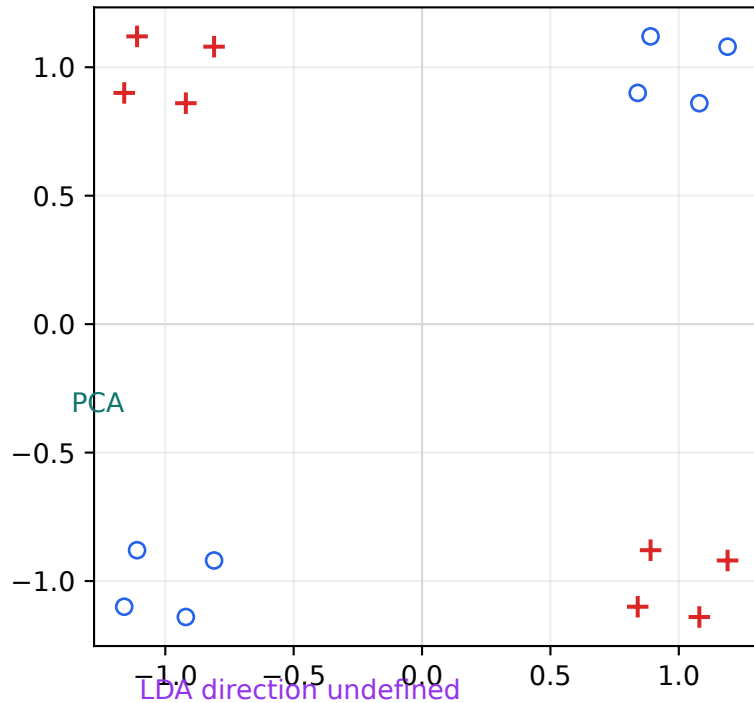
XOR: no good linear projection
